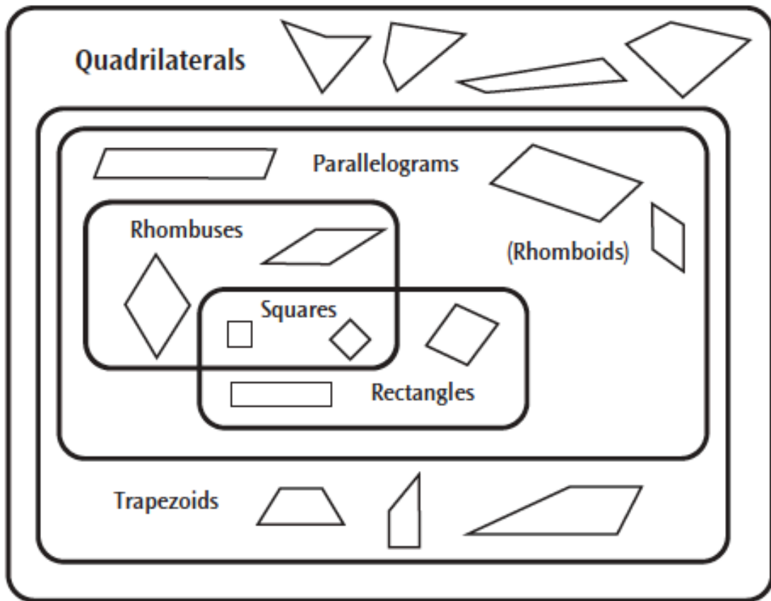
Figure 5-1. Classification of Quadrilaterals
