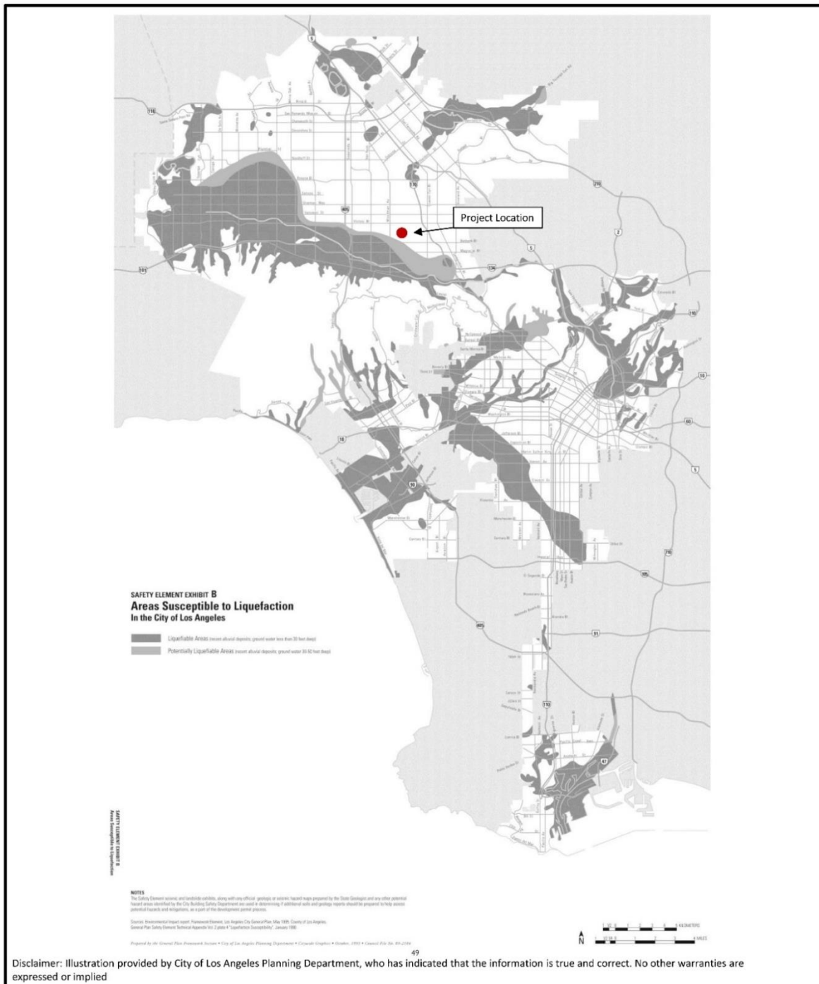
Figure 4.6-2 LIQUEFACTION ZONES
