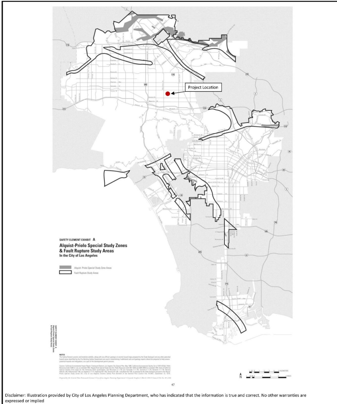
Figure 4.6-1 FAULT MAP
