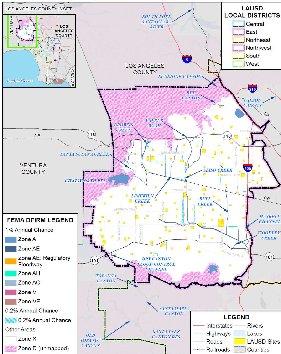
Figure 4-70 LAUSD – Local District Northwest DFIRM Flood Zones
