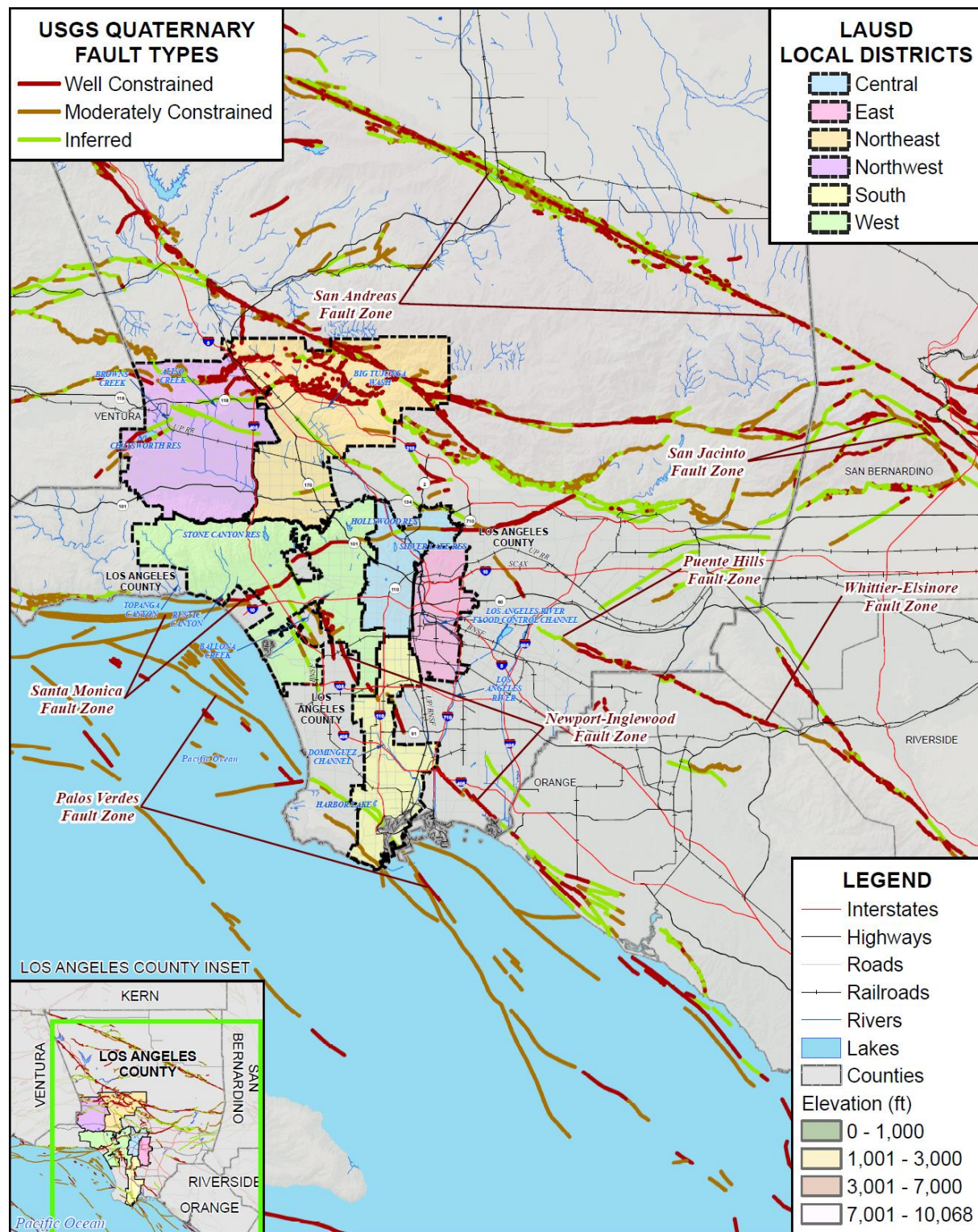
Figure 4-20 Active Faults in and near LAUSD
