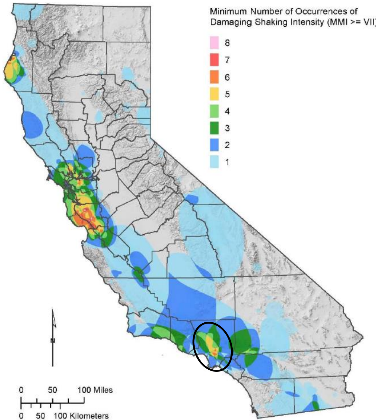
Figure 4-25 California Areas Damaged by Earthquake
