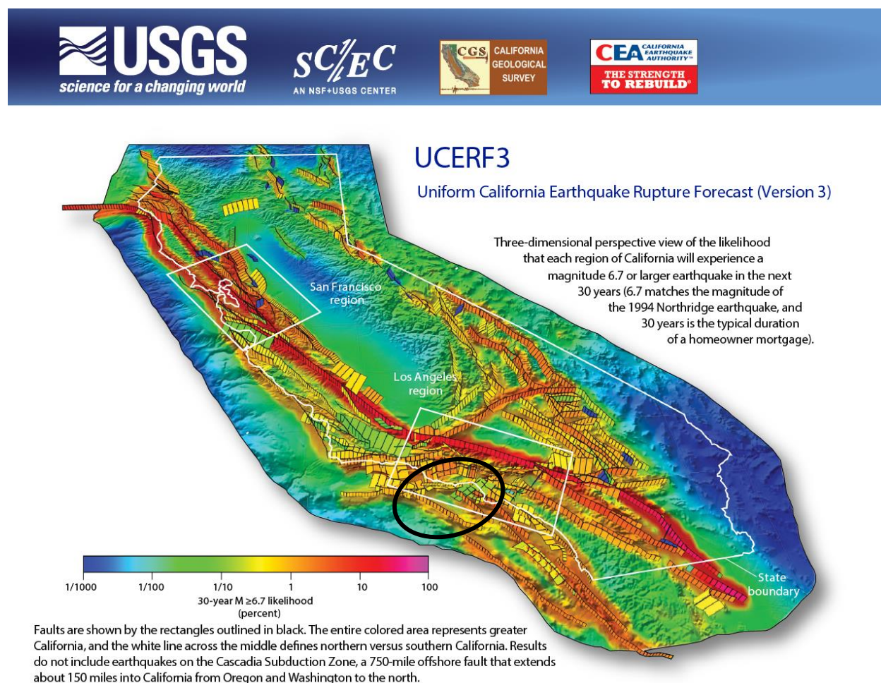
Figure 4-27 Probability of Earthquake Magnitudes Occurring in 30 Year Time Frame
