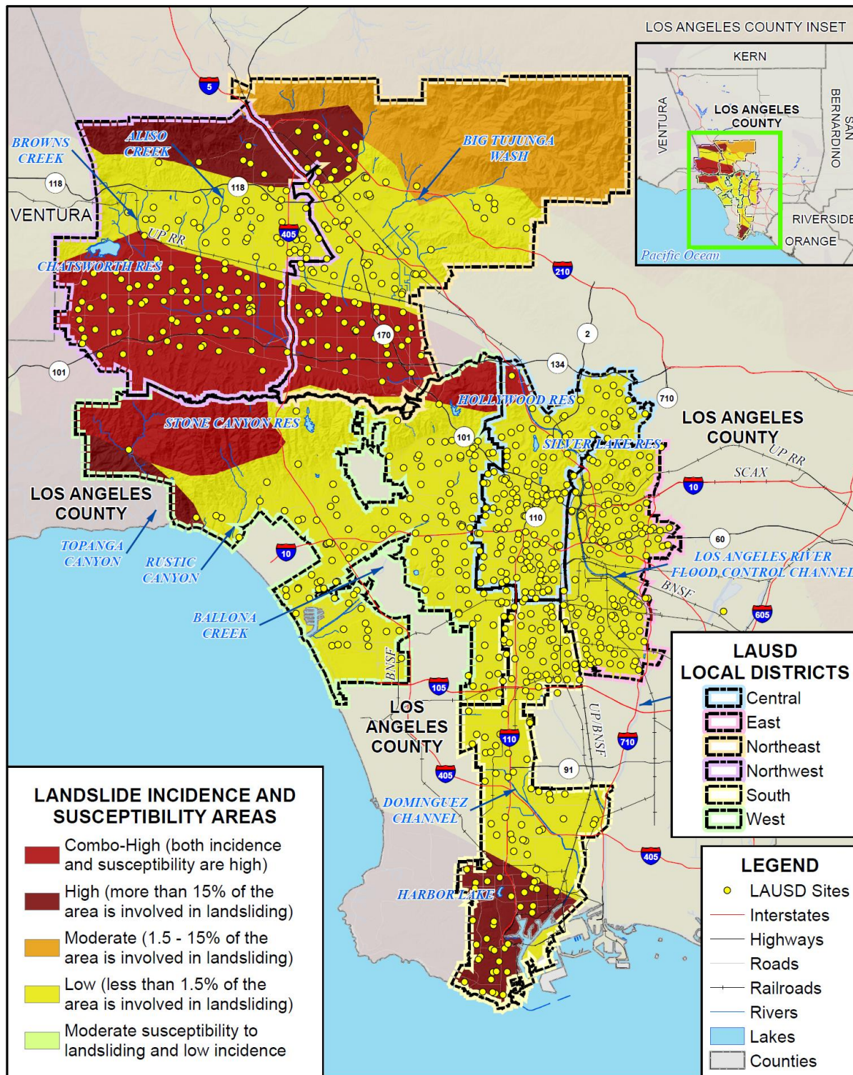
Figure 4-74 LAUSD – Landslide Incidence and Susceptibility Areas
