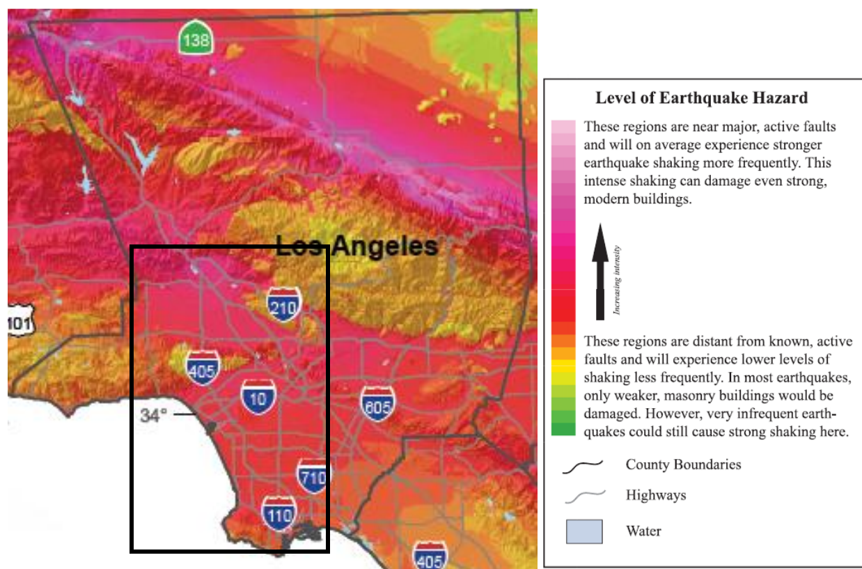
Figure 4-26 Maximum Expectable Earthquake Intensity – 2,500 Year Event
