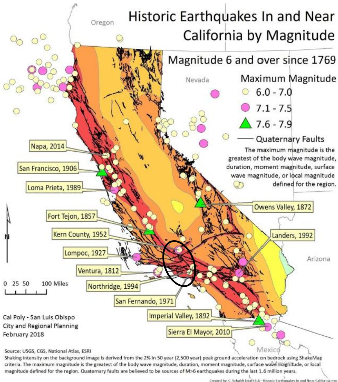
Figure 4-24 Historic Earthquakes in California (1769-2017)
