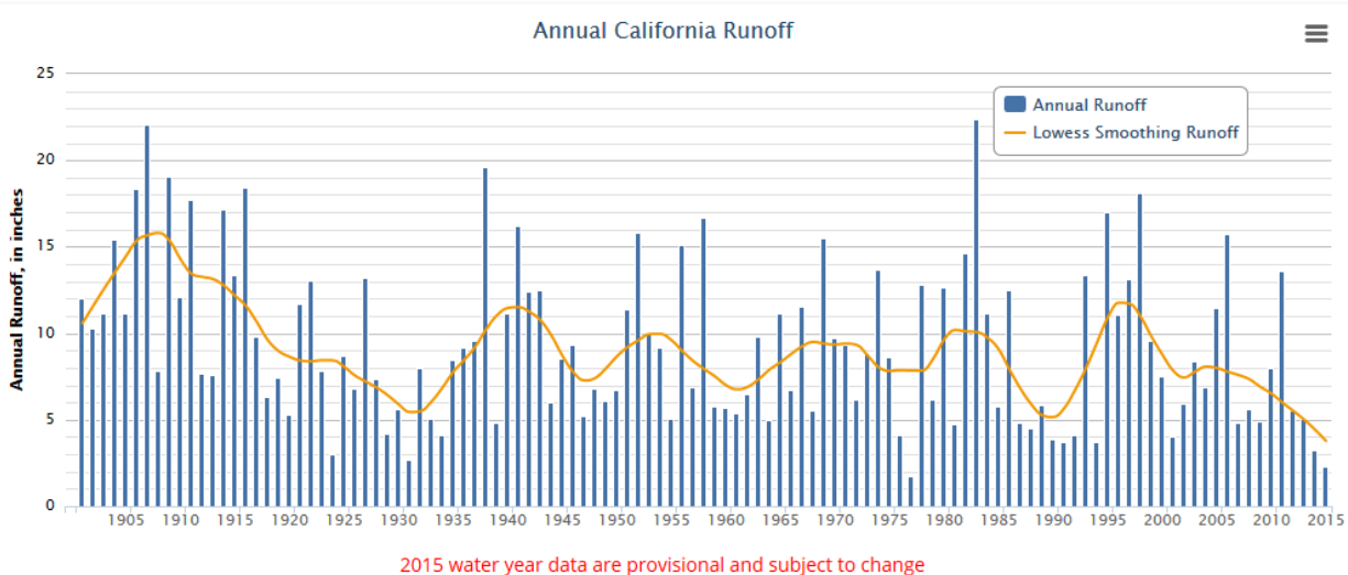
Figure 4-18 Annual California Runoff –1900 to 2015
