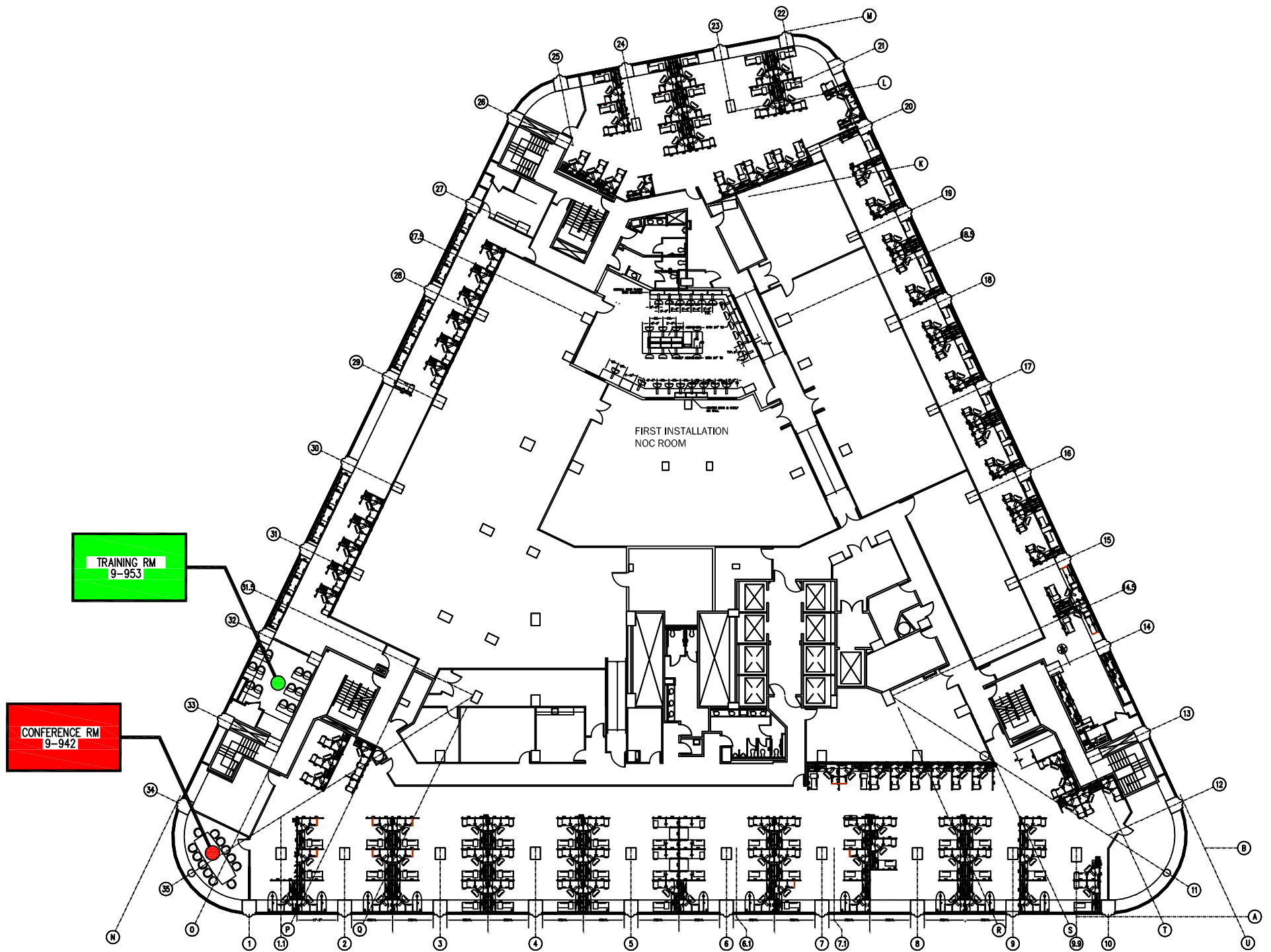
9th Floor Plan
